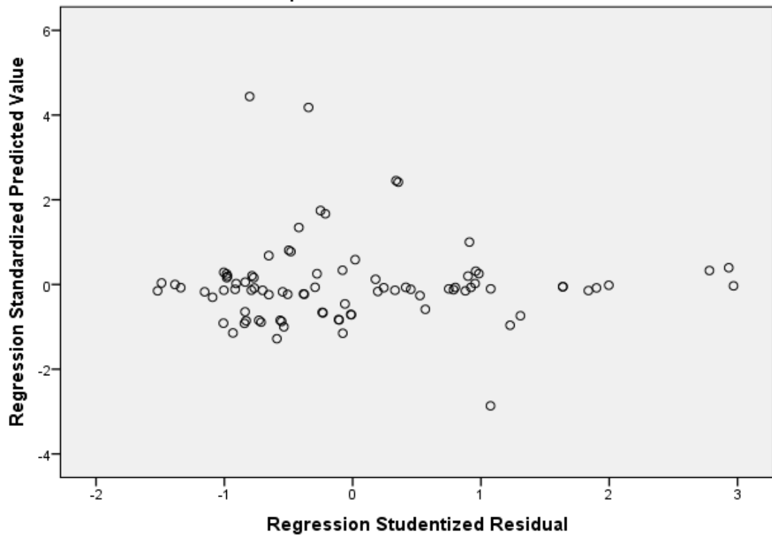
Scatterplot
